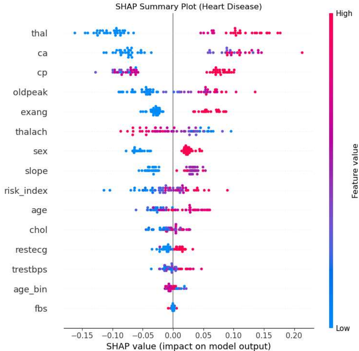
Step 3. Figure 5 – SHAP Summary Plot
